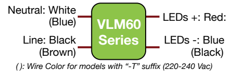
Wiring Diagram
