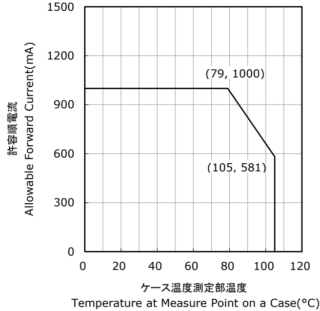
Temperature at Measure Point on a Case vs Allowable Forward Current
